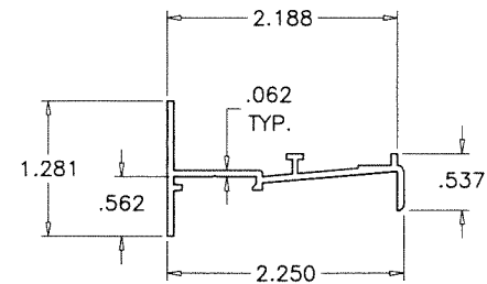
① FRAME HEAD/SILL
